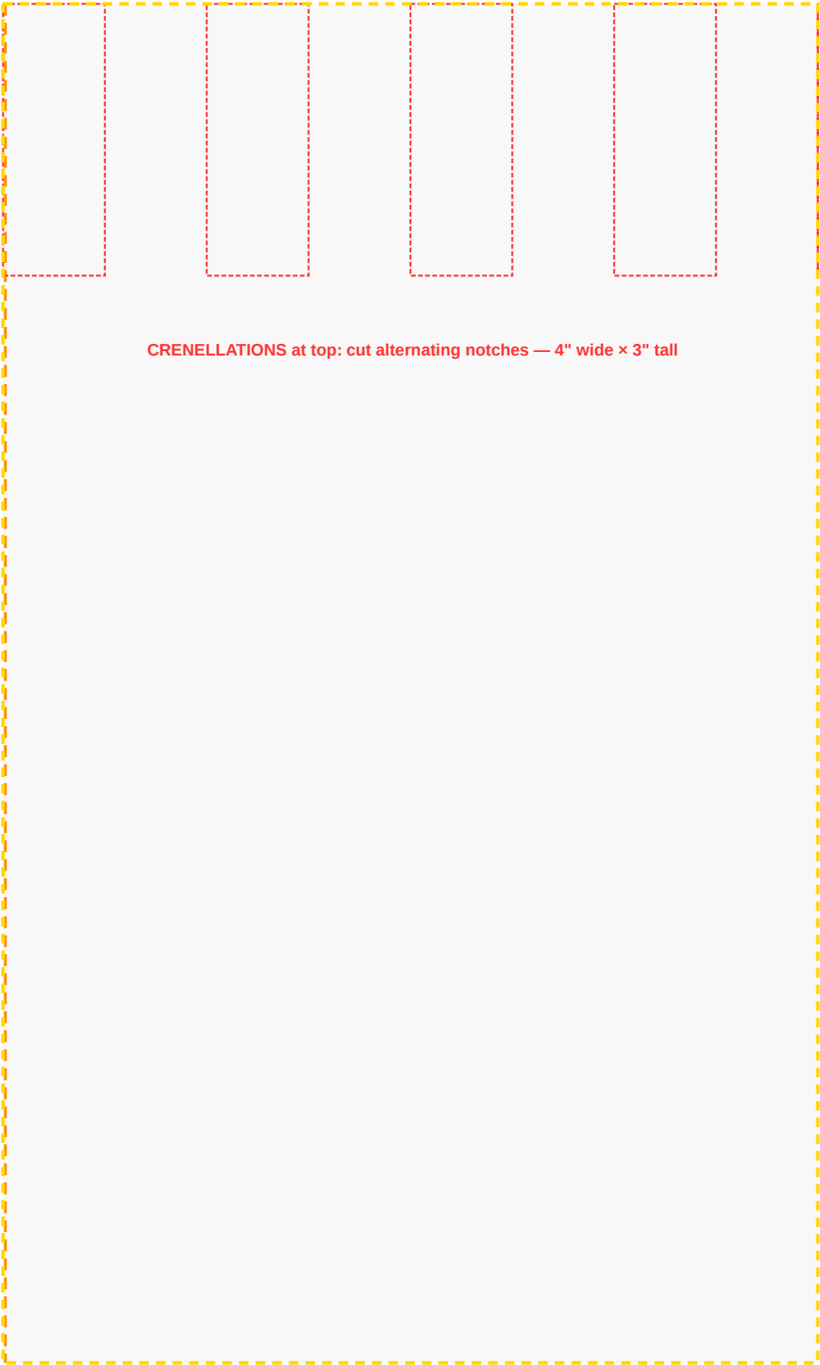
18" x 30" (46 x 76 cm) 2 panels per tower — tape at 90° corner
